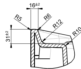
DETAIL B SCALE 0.400
