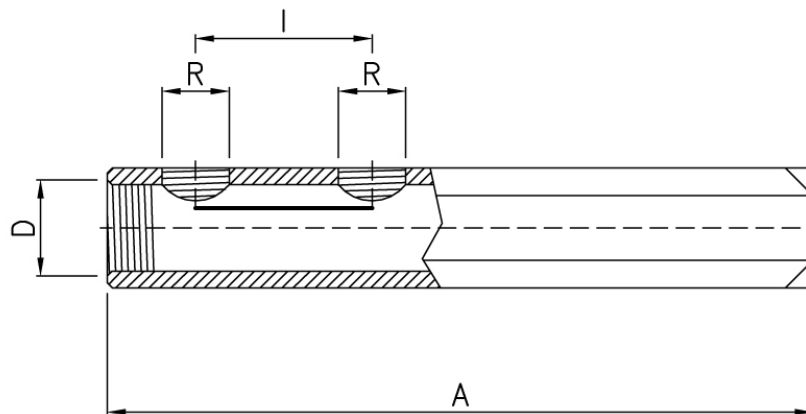
Collettori da barra - interasse 50 mm. Manifolds drawn - Center distance 50 mm.
